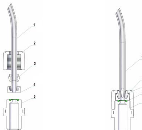
Fig.4 – Hydraulic Connection
